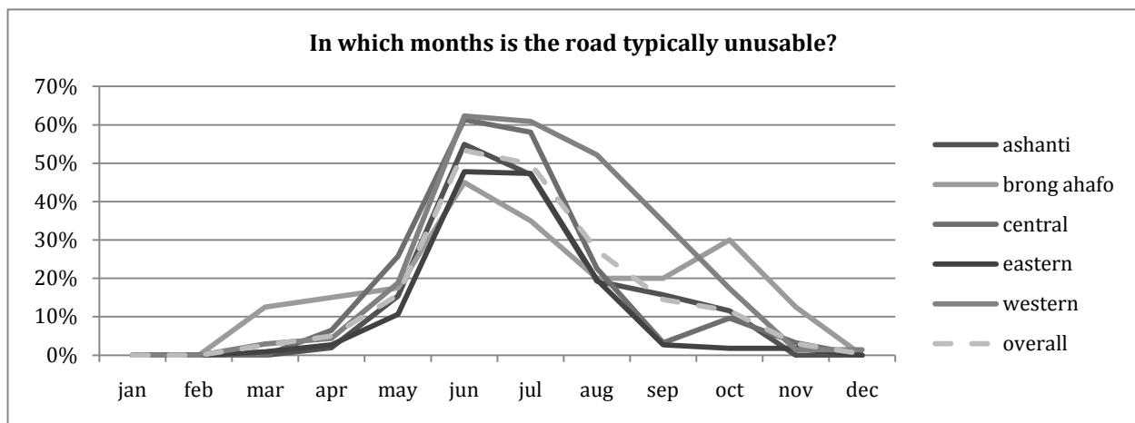
Figure 35: Road Conditions
